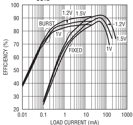
Efficiency vs Load Current and V_{IN} for V_{OUT2} = 1.8\text{V} at 1.2\text{MHz}
