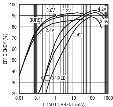
Efficiency vs Load Current and V_{IN} for V_{OUT1} = 5\text{V} at 1.2\text{MHz}
