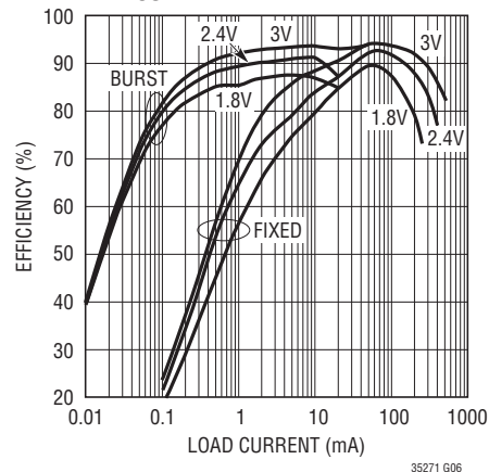
Efficiency vs Load Current and V_{IN} for V_{OUT2} = 3.3\text{V} at 2.2\text{MHz}
