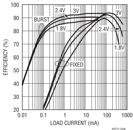
Efficiency vs Load Current and V_{IN} for V_{OUT1} = 3.3\text{V} at 2.2\text{MHz}
