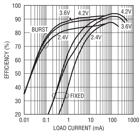
Efficiency vs Load Current and V_{IN} for V_{OUT2} = 5\text{V} at 1.2\text{MHz}
