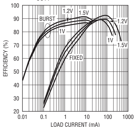
Efficiency vs Load Current and V_{IN} for V_{OUT1} = 1.8\text{V} at 1.2\text{MHz}
