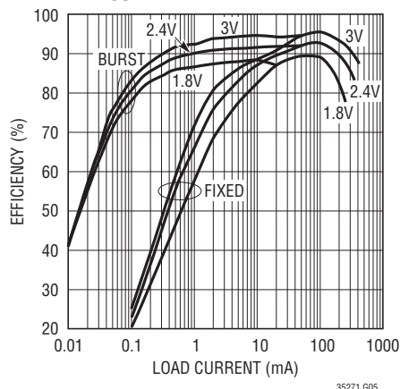
Efficiency vs Load Current and V_{IN} for V_{OUT2} = 3.3\text{V} at 1.2\text{MHz}
